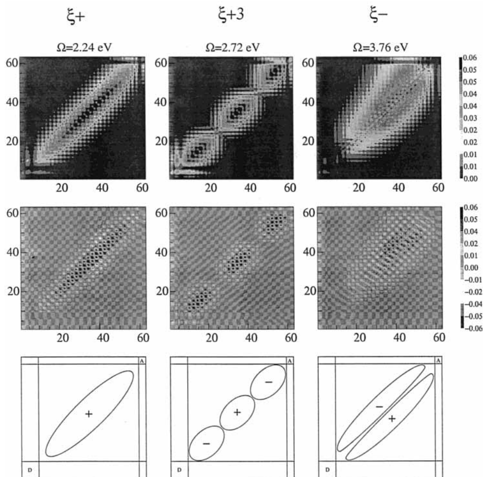
Figure 7. \xi_+ , \xi_{+3} , and \xi_- oscillators of CAR(25). Upper row, \xi_{mm} in the atomic basis set; middle row, \xi_{mm,PzPz} ; bottom row, illustration of symmetry properties.
